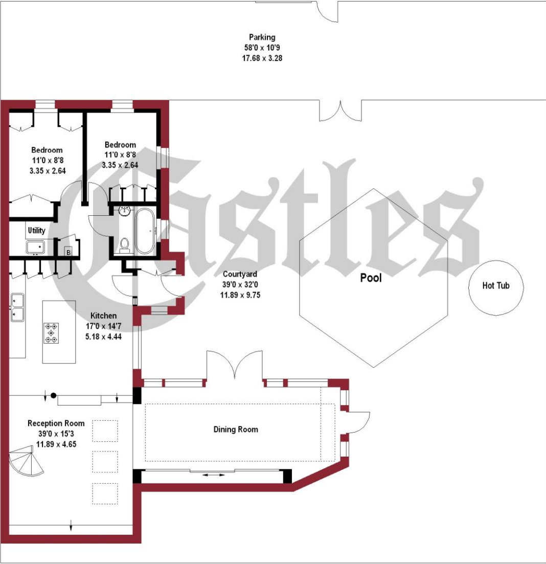
GROUND FLOOR
